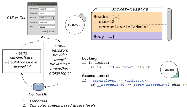
Figure 5: Illustration of the access control system.
